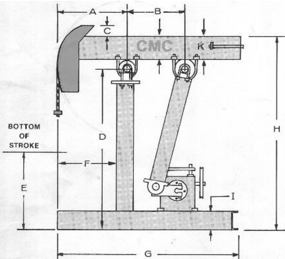
GENERAL DIMENSIONS OF PUMPING UNITS
