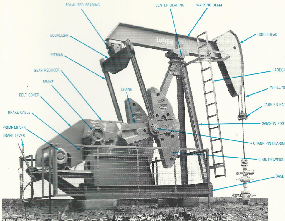
FIGURE 26 Conventional Pumping Unit Nomenclature
