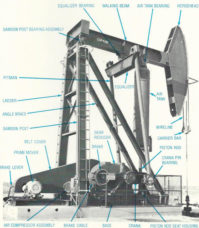
FIGURE 27 Air Balanced Pumping Unit
