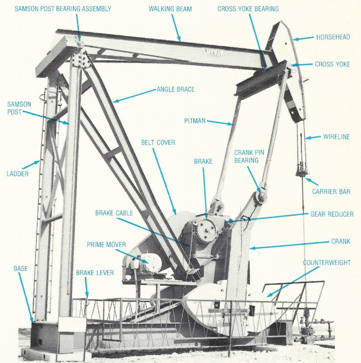
FIGURE 28 Mark II Pumping Unit
