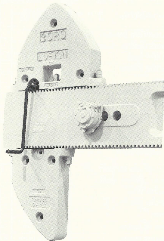
FIGURE 13—illustrating the wide range of counterweight sizes which can be used on one crank. Different size counterweights are not normally furnished or recommended for the same unit.
